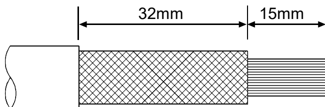
Double Insulated (25mm 2 )
